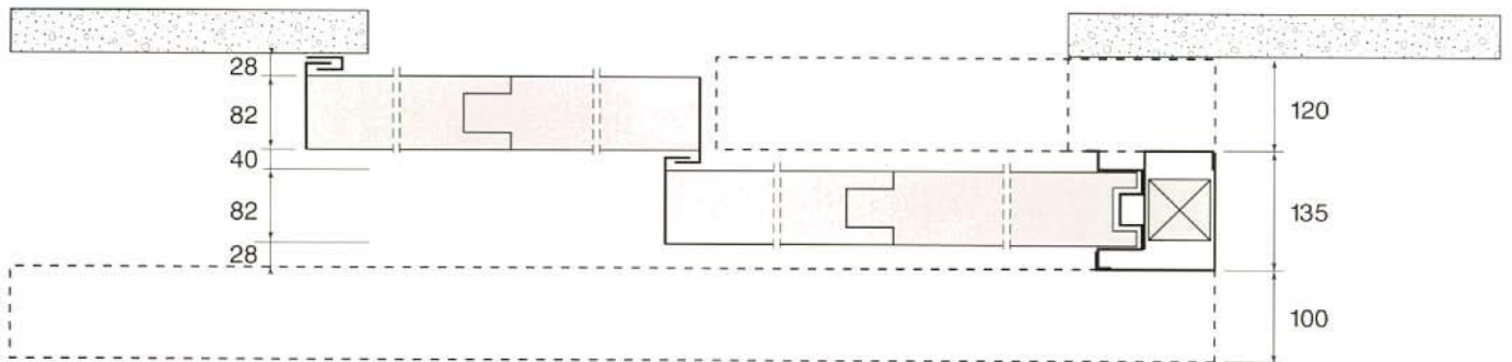
Sec. BB
