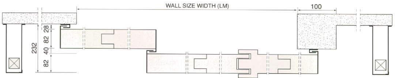
Sec. BB
