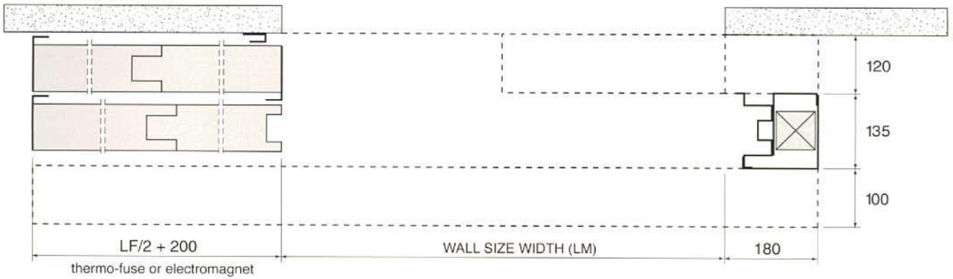
Sec. BB
